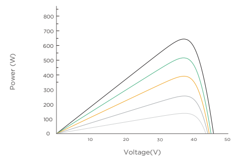
I-V/P-V Curve at Different Temperature (700W)
